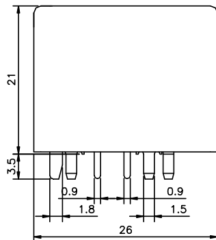
ETR CAR–SS/SH (Europe)
