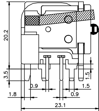
ETR CAR (Open Type—U.S.A.)
