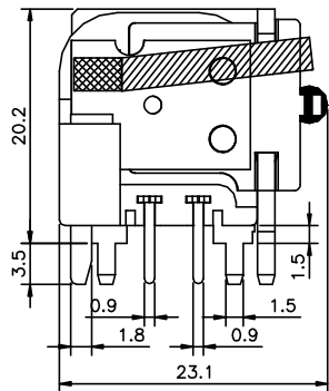
ETR CAR (Open Type–Europe)
